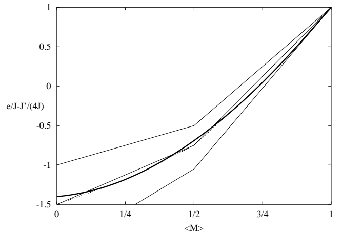
Fig. 2. Ground state energy per site versus magnetization. Bold line: Spin-1 chain equation (2.3). Thin lines: equation (2.2) for J'/J = 1, 1.5 and 2.1 (from top to bottom). Dashed lines: Maxwell constructions required for J'/J = 1.5 .
