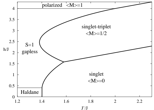
Fig. 4. Ground state phase diagram for the two-leg ladder. The heavy lines denote first order transitions, the thin ones second order transitions.
