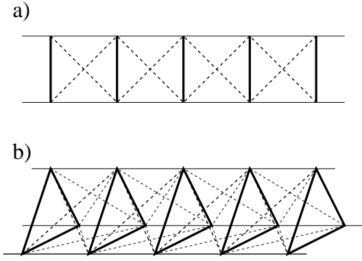
Fig. 1. Geometry of the (a) two-leg and (b) three-leg ladders considered in the present paper. The thick full lines denote coupling J' , the thin full lines coupling J and the dashed lines coupling J_\times . Throughout this paper we use J = J_\times .
