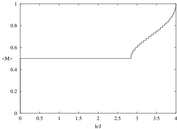
Fig. 5. Magnetization curve of the S = 3/2 - 1/2 ferrimagnetic chain for L = 60 .
