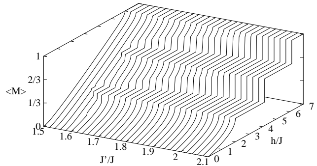
Fig. 6. Magnetization curves of the three-leg ladder (Eq. (1.1)).
