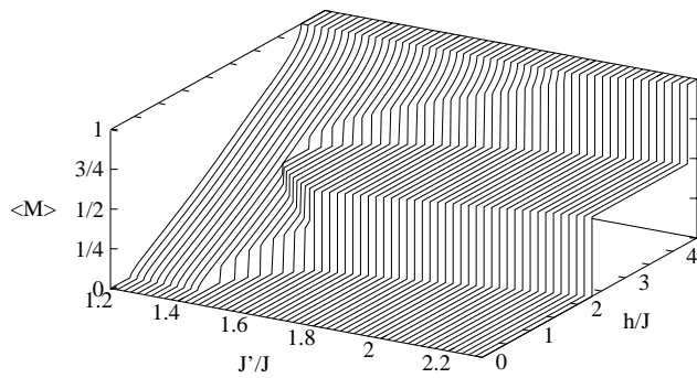
Fig. 3. Magnetization curves of the two-leg ladder equation (1.1).
